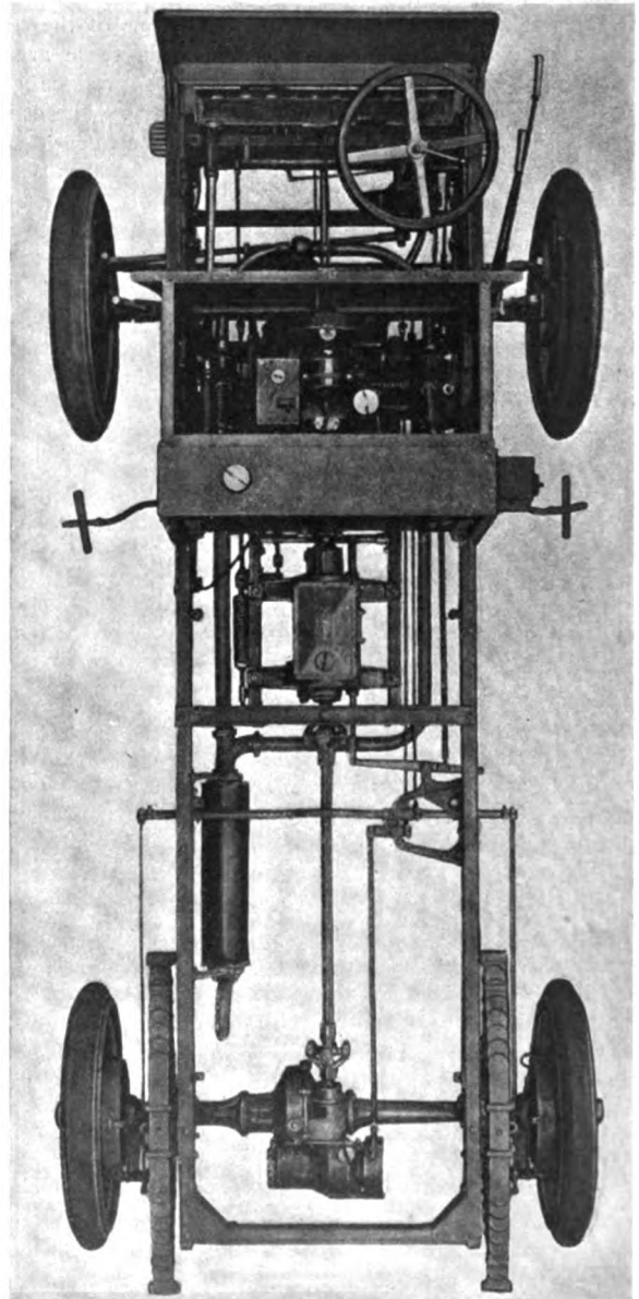
Autocar Company Features a Utility Chassis.
